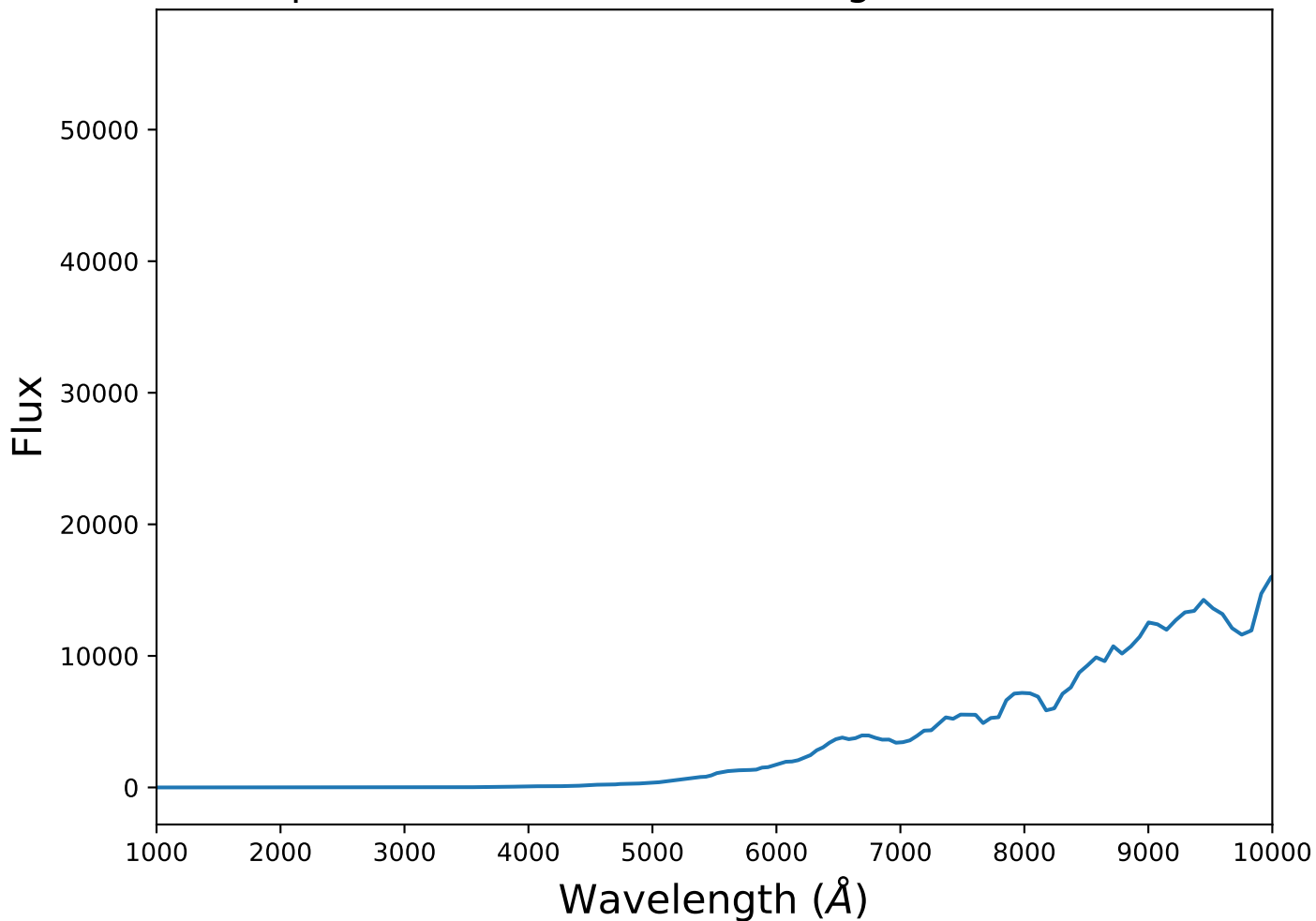
Spectrum 6 for transient 91bg-like at z=0.23
